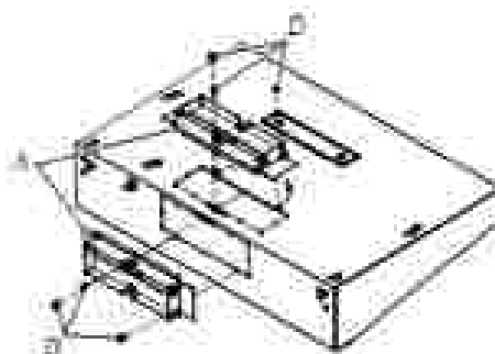
A. 24" x 10" (61.3 x 25.4 cm) rectangular vent damper B. 3.5 x 9.5 mm screws
