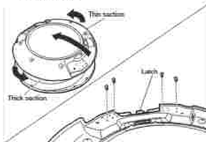
Figure 6 • Remove latch
