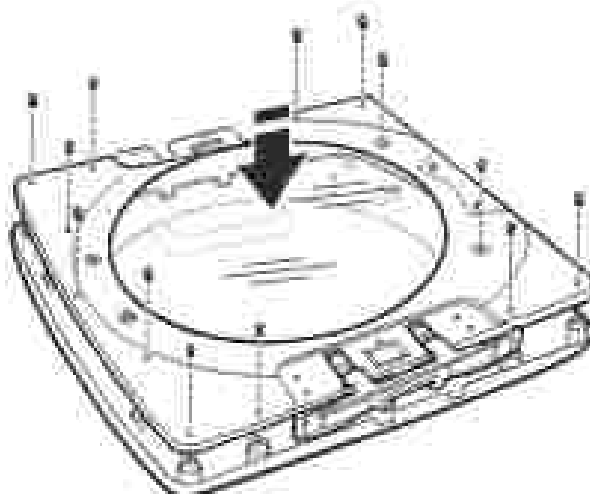
Figure 5 - Reattach inner door to outer door.
