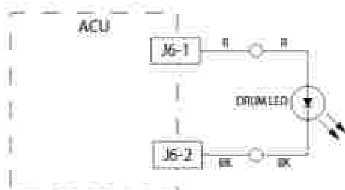
Figure 2 - Drum LED Schematic Circuit
