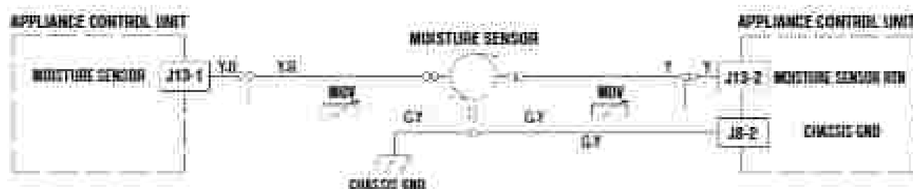
Figure 3 • Moisture Sensor Strip Circuit
