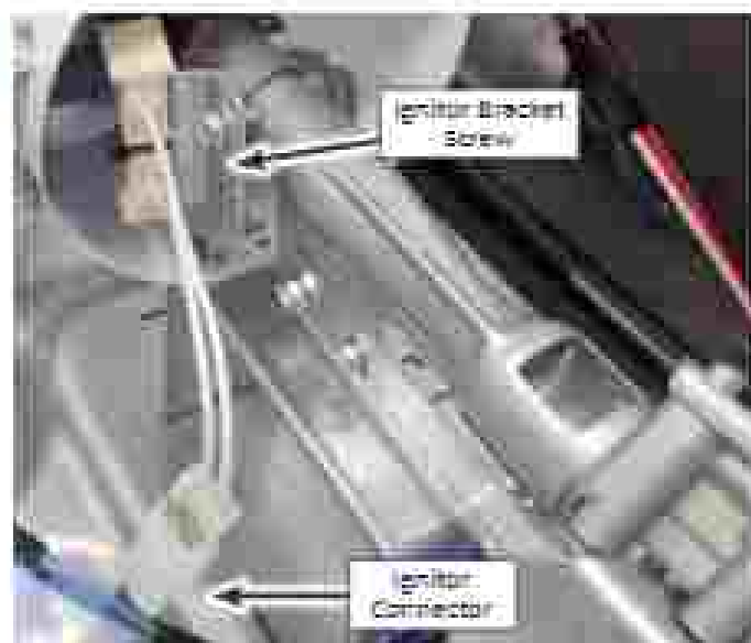
Figure 2 - Removing Ignitor
