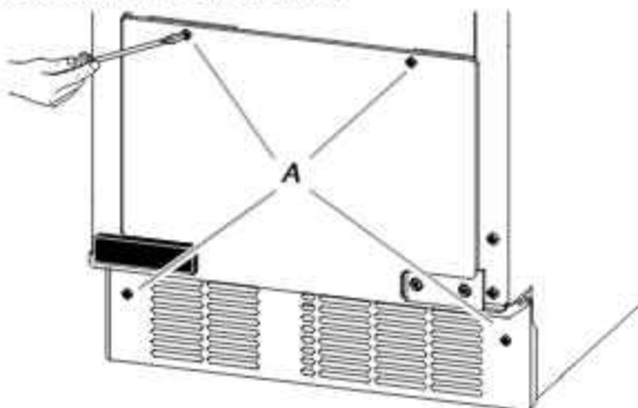
A. Grill cover screws
