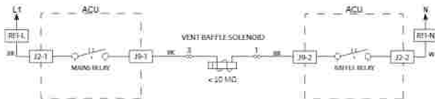
Figure 3 – Vent Baffle Solenoid Wiring Circuit
