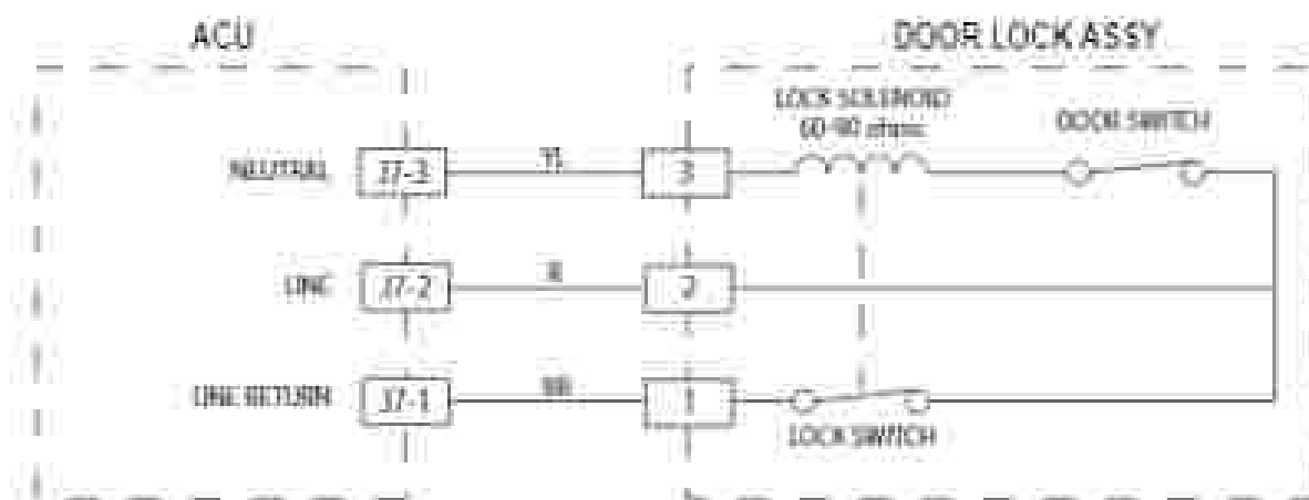
Figure 2 - Door Lock Wiring Chart
