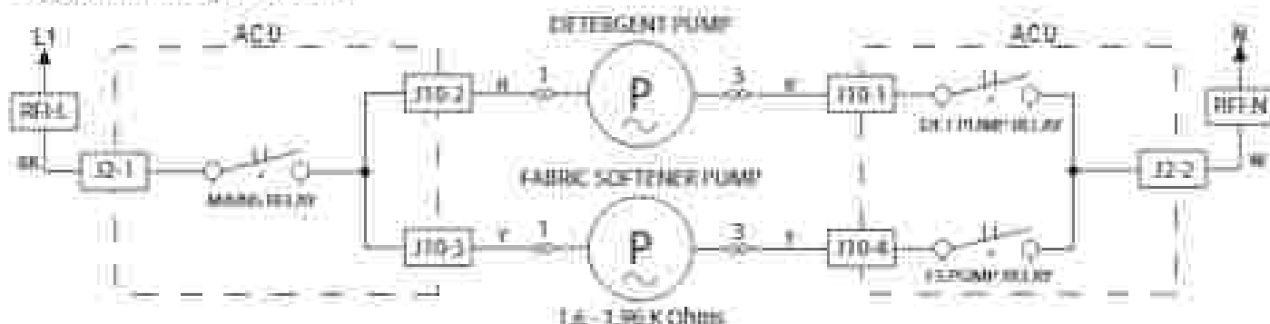
Figure 1 - Detergent Dosing Pump Wire Circuit
