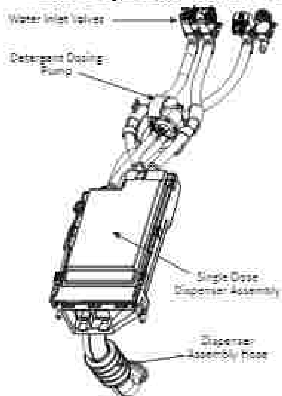
Figure 2 - Optimal Dispenser - Dosing Pump Location
