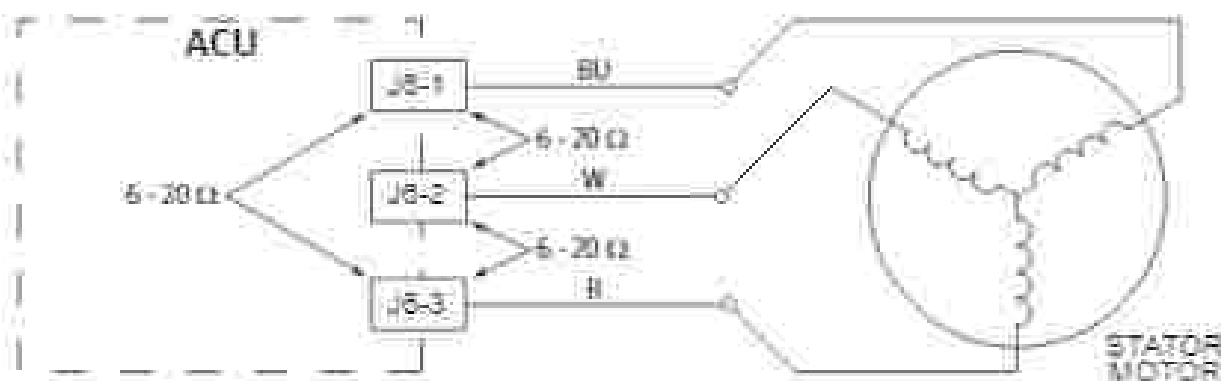
Figure 2—Direct Drive Motor Wire Circuit
