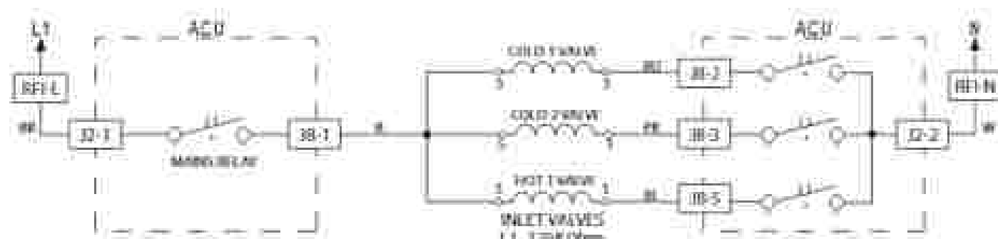
Figure 2 - Inlet Water Valves Step Circuit
