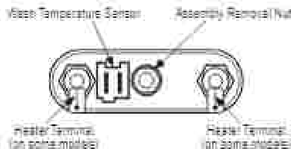
Figure 2 - Heating/Temperature Sensor Assembly
