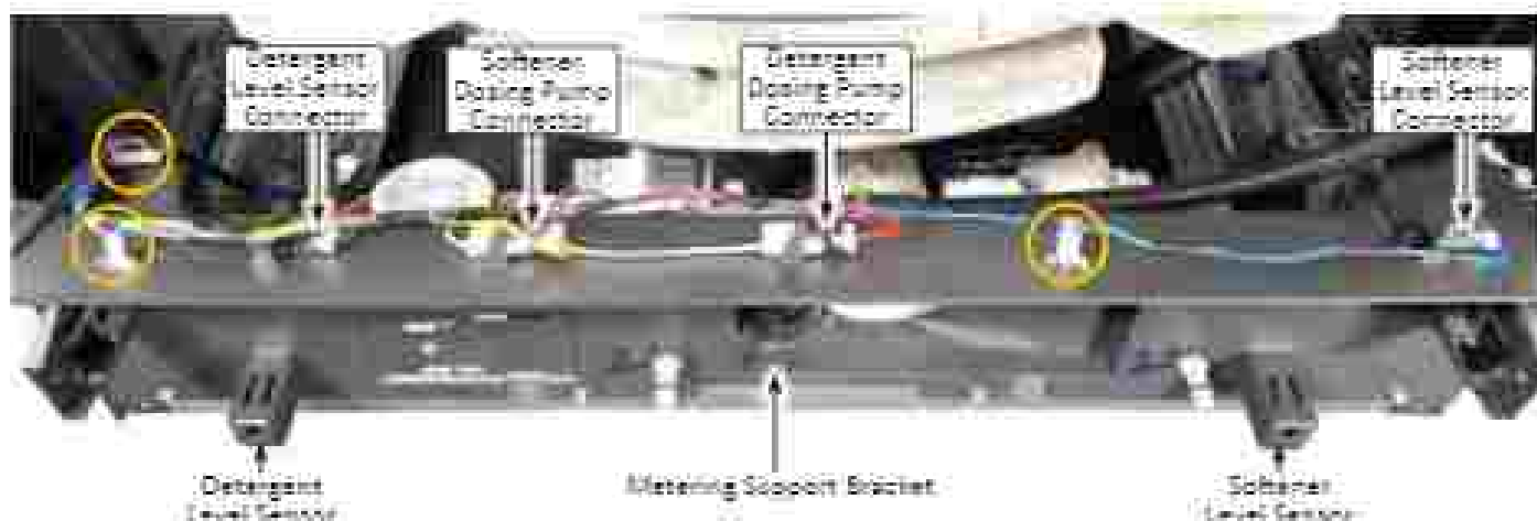
Figure 4 - Bulk Dispense Assembly
