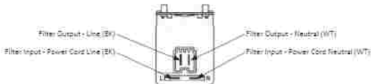
Figure 3 - Electrical Connections
