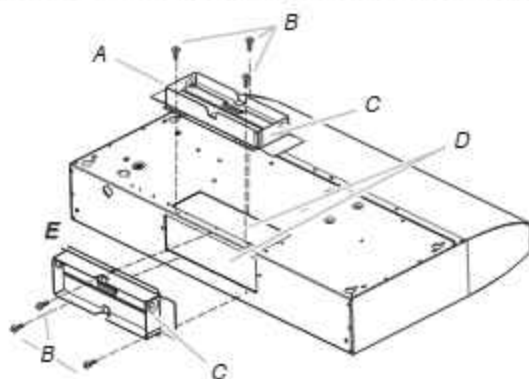
A. Vertical vent D. Vent knockouts B. Sheet metal screws E. Horizontal vent C. Hinge pin
