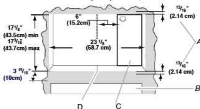
A. Trim kit frame overhang B. Cutout for lower oven C. Recommended region for receptacle location (no less than 6" [15.2 cm] to the right of cutout centerline) D. Cutout centerline
