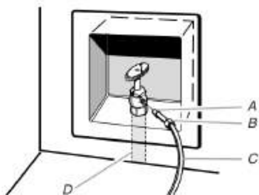
A. Bulb B. Nut C. Copper or PEX tubing (to refrigerator) D. Household supply line (½" minimum)
