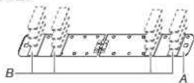
A. Mounting plate B. 1/16" thickness Spacer
