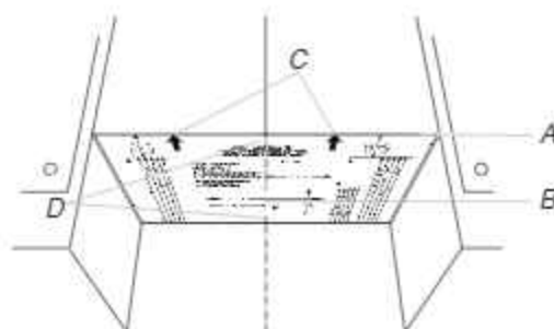
A. Front Edge of the Upper Cabinet Template and Front Edge of Upper Cabinet B. Upper Cabinet Centerline C. Arrows on Upper Cabinet Template D. Center Marks on Upper Cabinet Template
