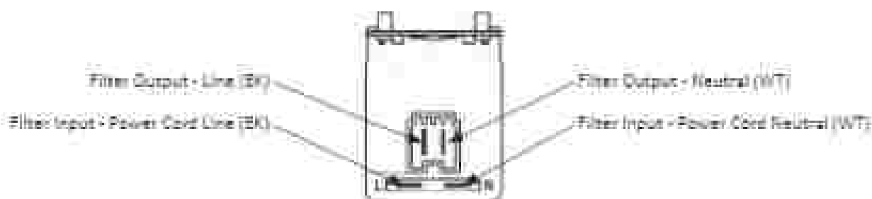
Figure 3 • Electrical Connections
