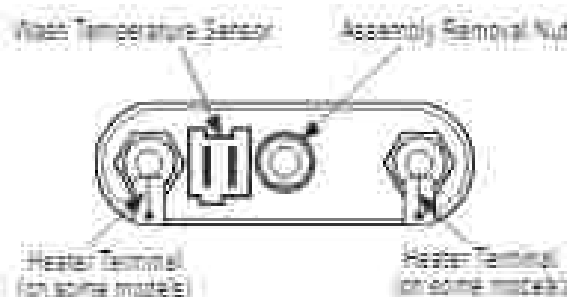
Figure 2 - Wash Temperature Sensor
