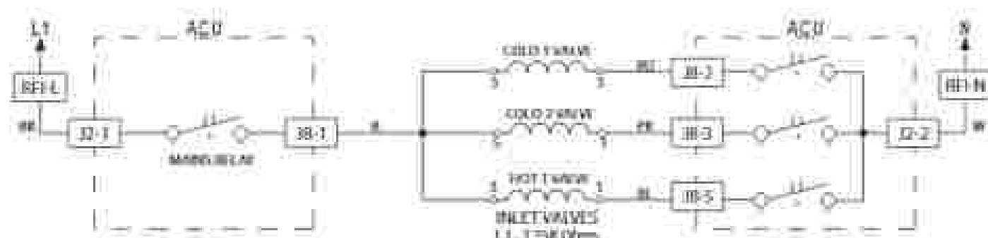
Figure 2 - Inlet Water Valves Stop Circuit
