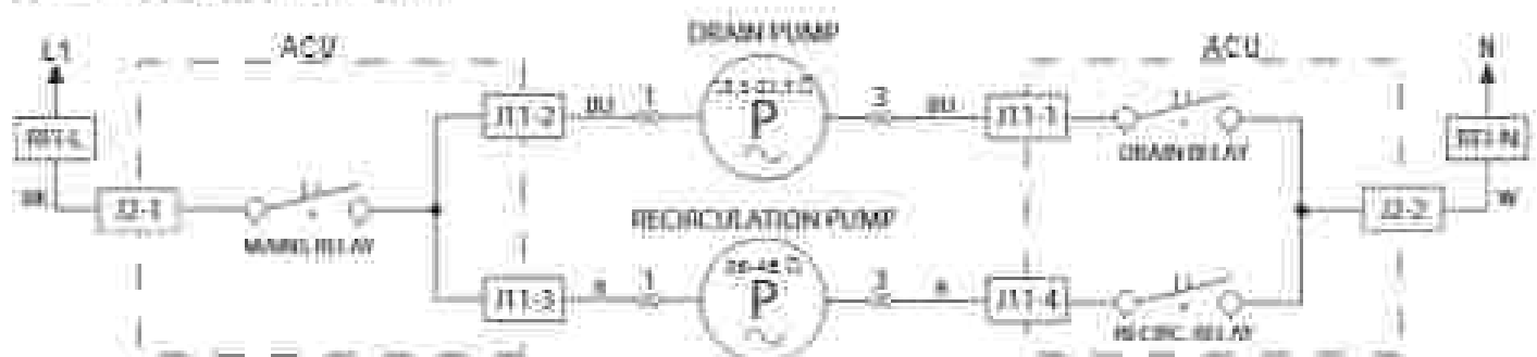
Figure 3 - Drain/Recirculation Pump Wiring Circuit
