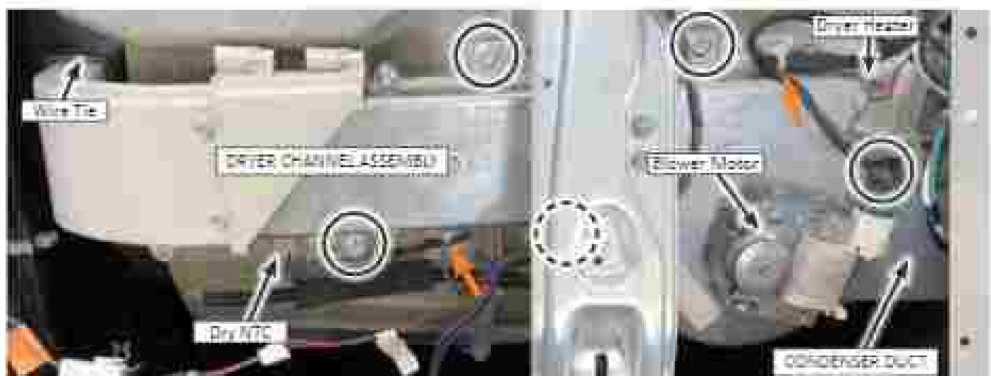
Figure 4: Dryer Channel Assembly
