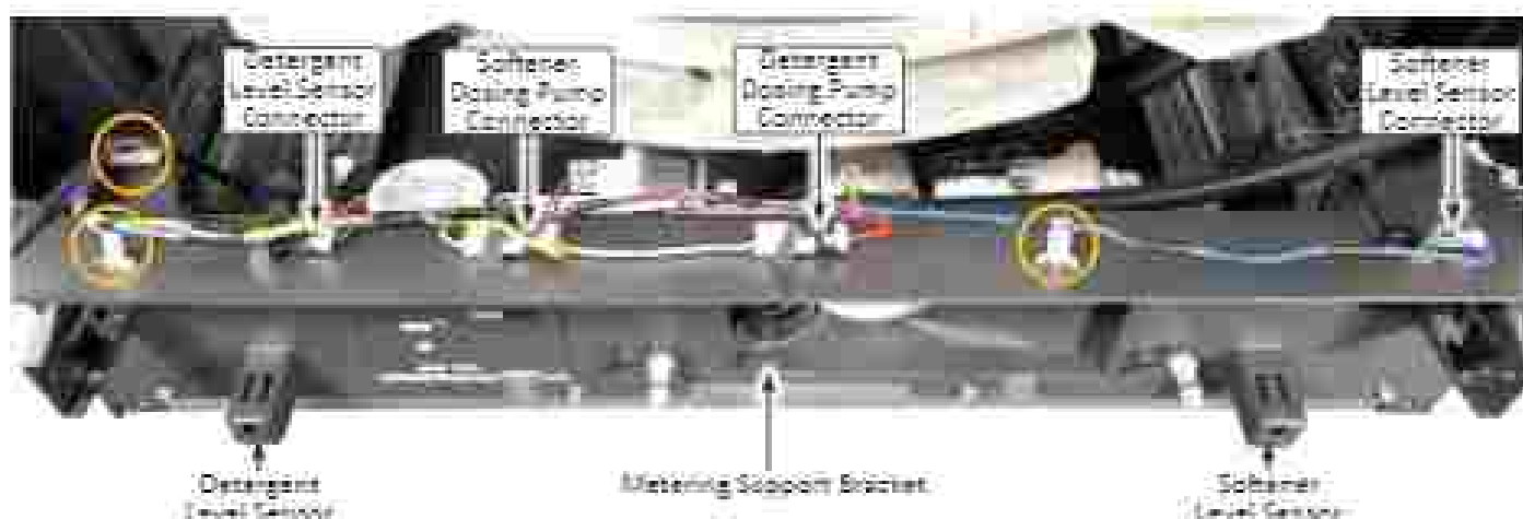
Figure 1 - Bulk Dispense Assembly
