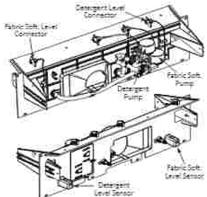
Figure 1—Drawer Bulk Dispenser Components
