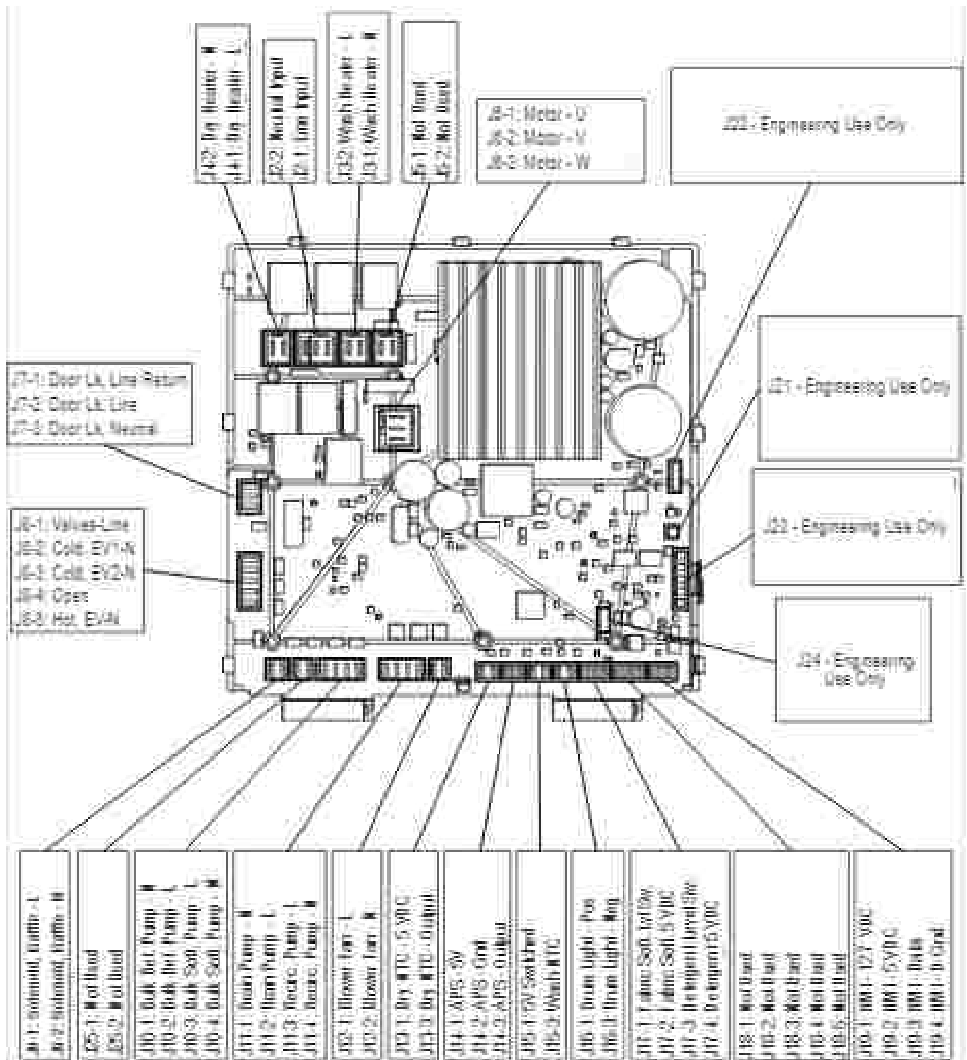
ACU CONNECTORS &amp; PINOUTS - FIGURE 2
