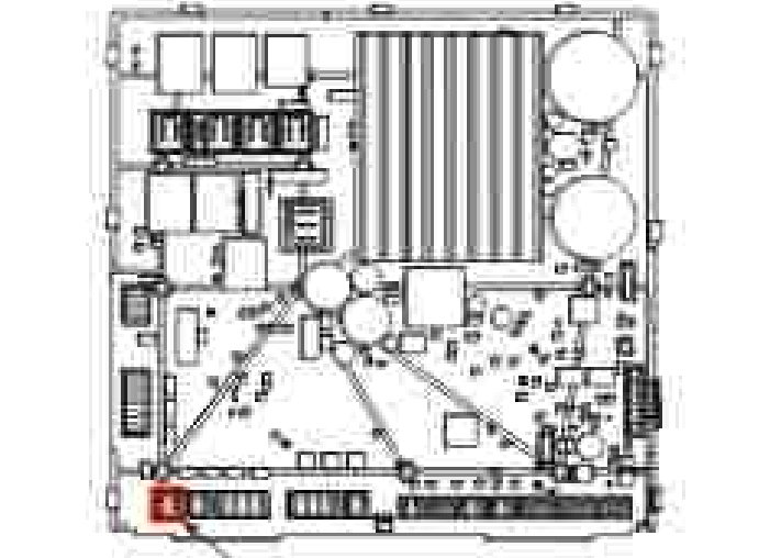
Figure 2—Location of Baffle Solenoid Connector on ACU
