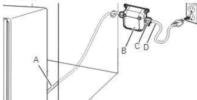
A. Junction box cable B. Junction box C. Cable fittings (2) D. Power cord
