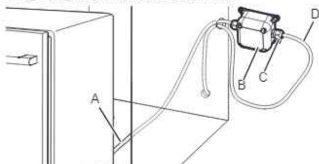
A. Junction box cable B. Junction box C. Cable fittings (2) D. Home wiring
