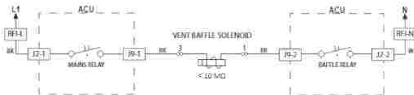
Figure 3 - Vent Baffle Solenoid Strip Circuit
