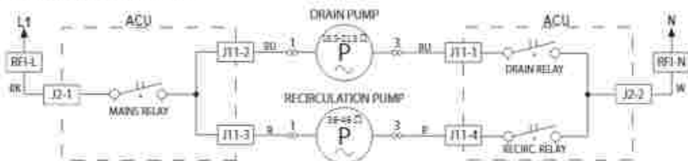
Figure 2 - Drain/Recirculation Pump Strip Circuit
