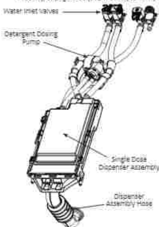
Figure 1 - Optimal Dispense - Dosing Pump Location
