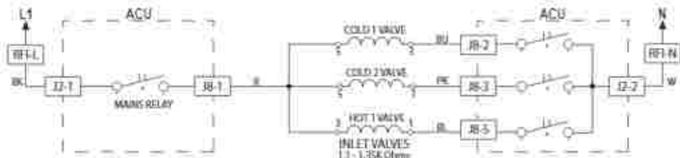
Figure 2 - Inlet Water Valves Strip Circuit
