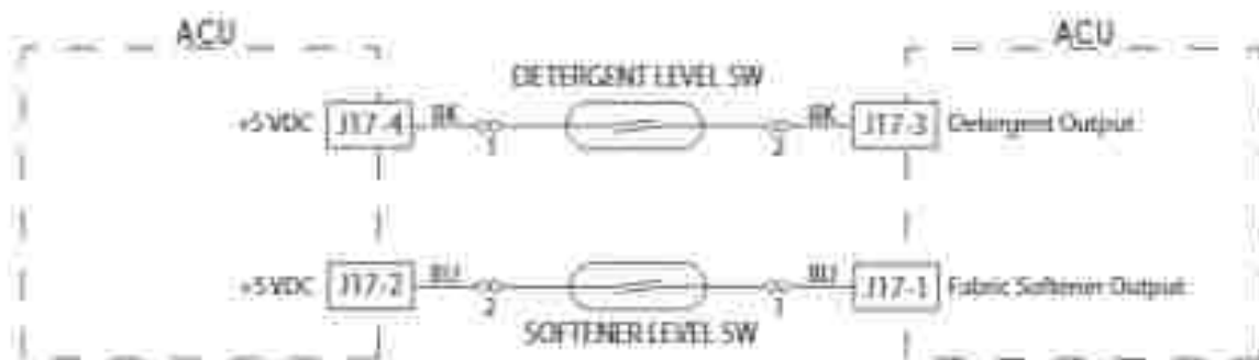
Figure 2 - Bulk Dispense Level Sensing Strip Circuit
