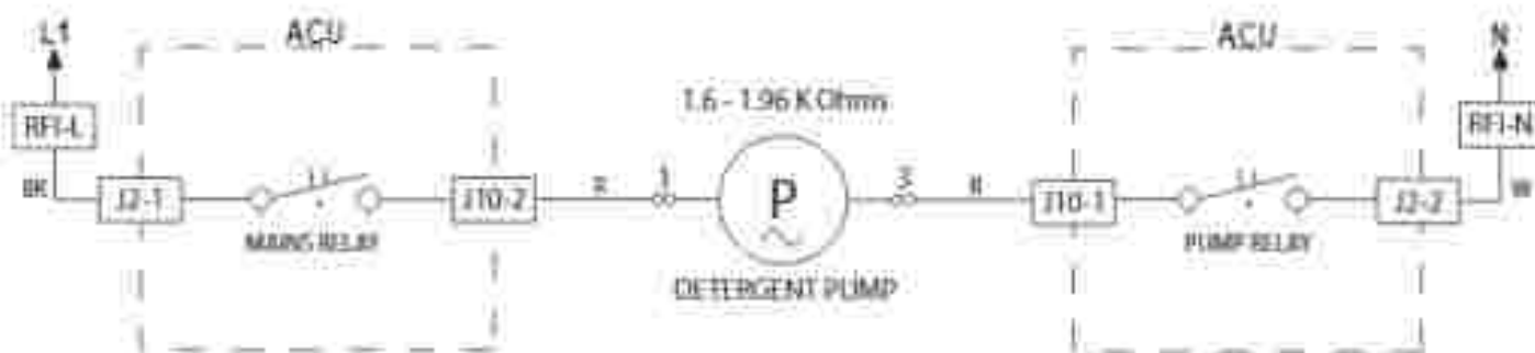
Figure 2 - Detergent Dosing Pump Strip Circuit
