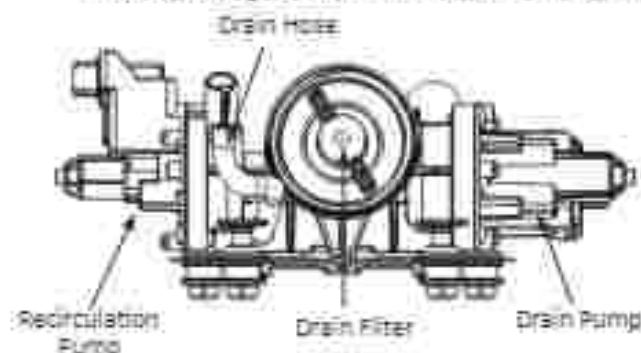
Figure 1 - Drain/Recirculation Pump
