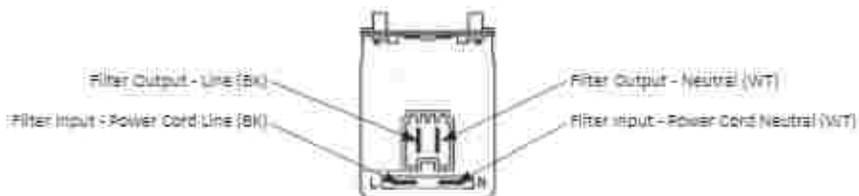
Figure 3 - Electrical Connections
