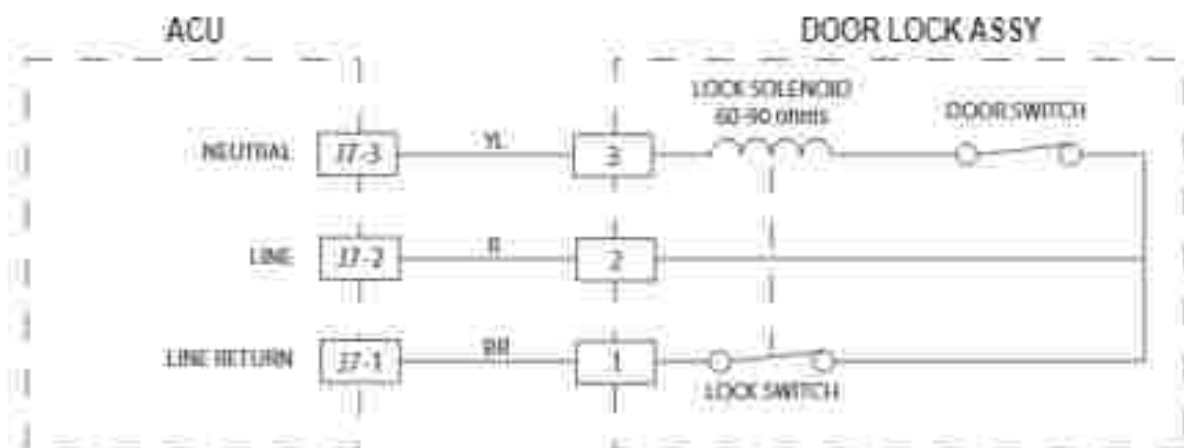
Figure 3 - Door Lock Sump Circuit
