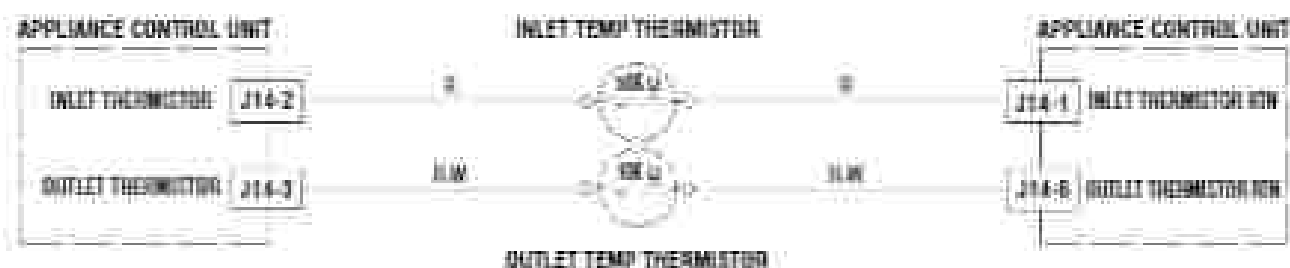
Figure 1 • Thermistors Strip Circuit (Resistance values shown at relative room temp.)
