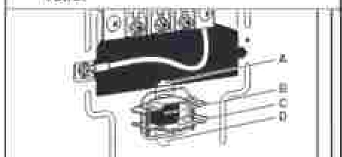
4-wire receptacle (NEMA type 14-30F)
