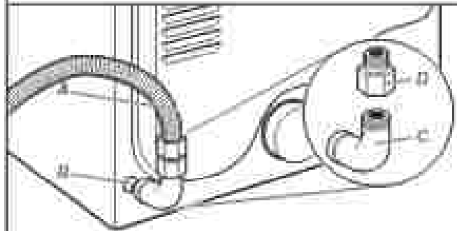
A. 3/8" flexible gas connector C. 3/8" to 3/8" pipe elbow B. 3/8" dryer pipe D. 3/8" pipe-to-fan adapter fitting
