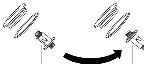
A. Propane gas position B. Natural gas position
