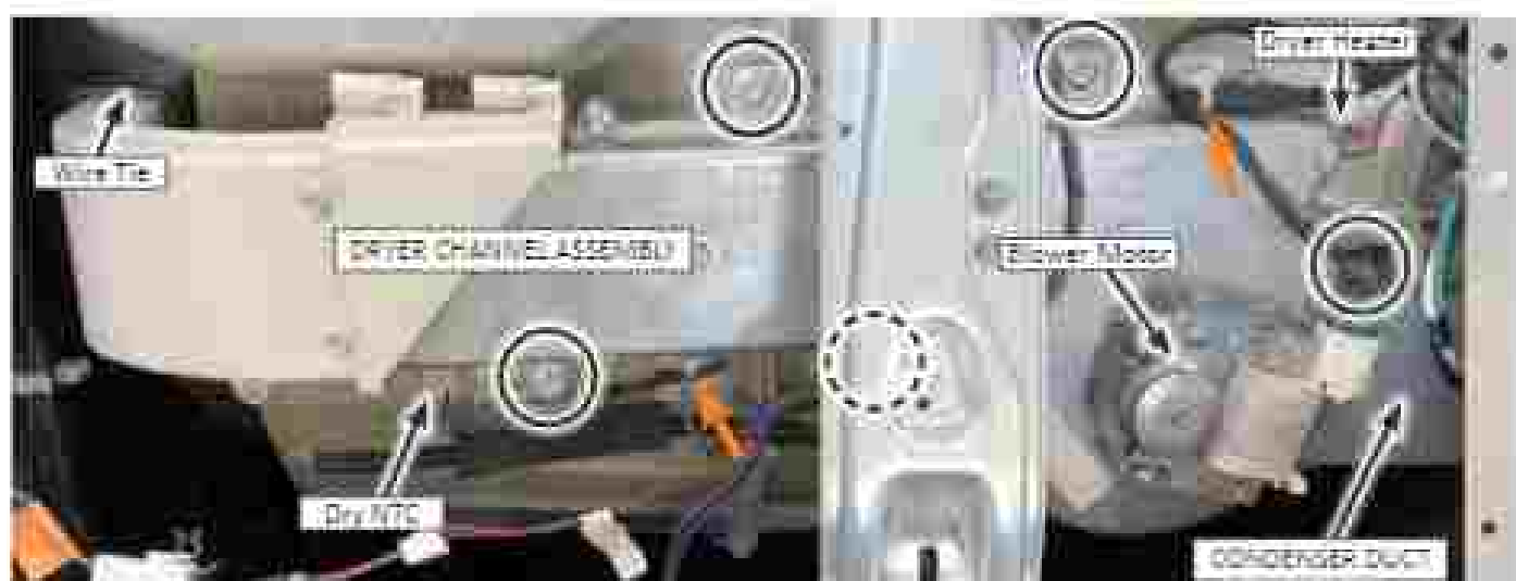
Figure 4: Dryer Channel Assembly
