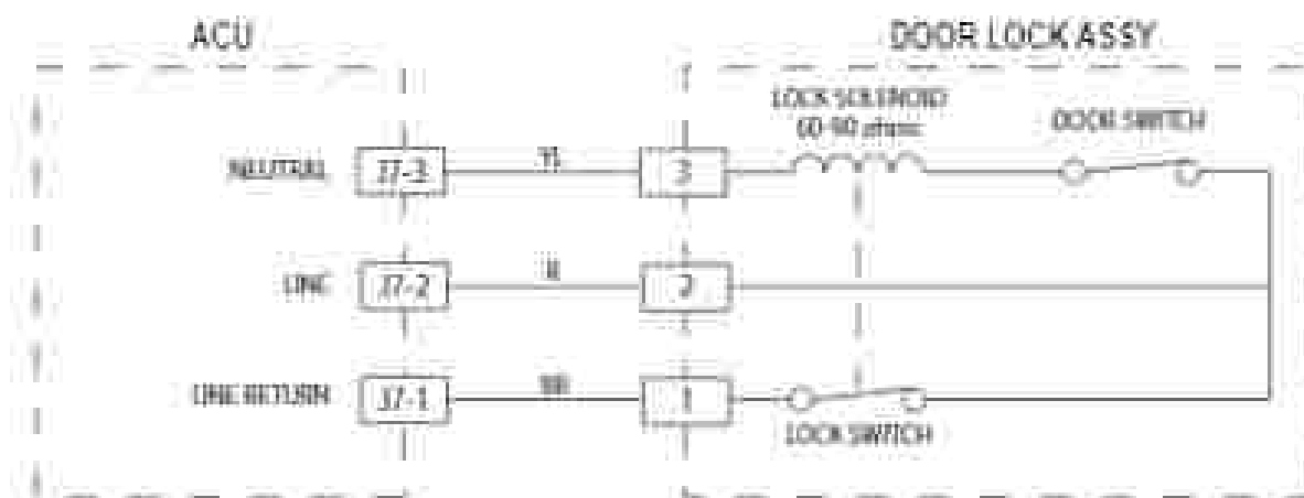
Figure 2 • Door Lock Strip Circuit
