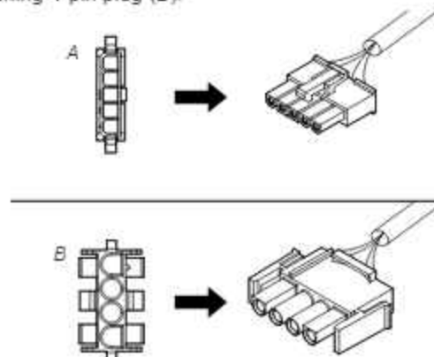
Determining the proper jumper
