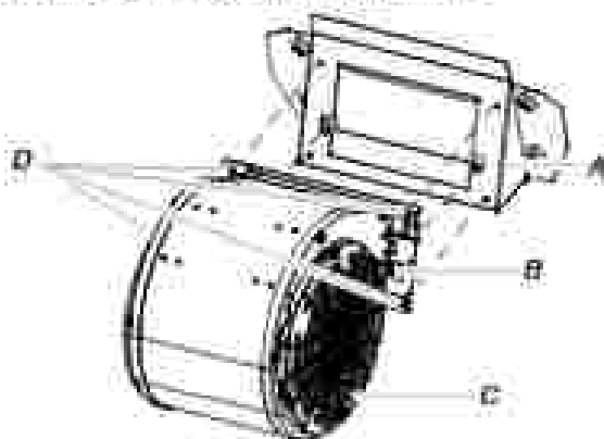
A. Rear motor mounting bracket B. Motor mounting tabs (4) C. Blower motor D. Blower motor mounting screws (4)
